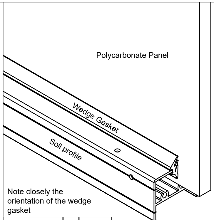
Simplified Drawing
