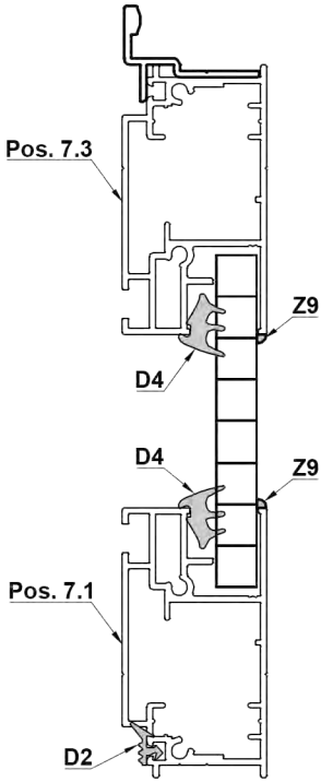
Detail B-B
