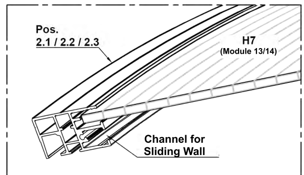
Detail B
