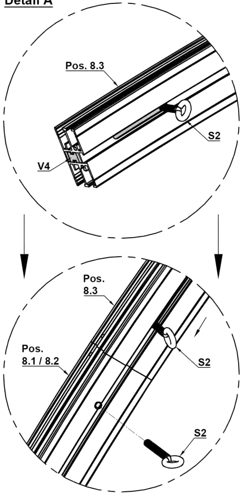
Detail A
