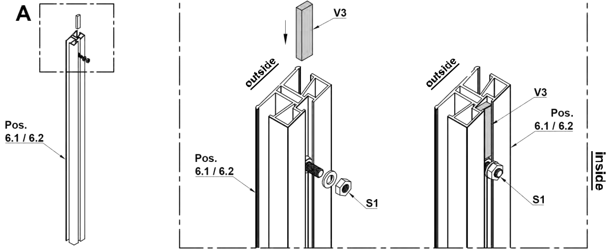
Detail A
